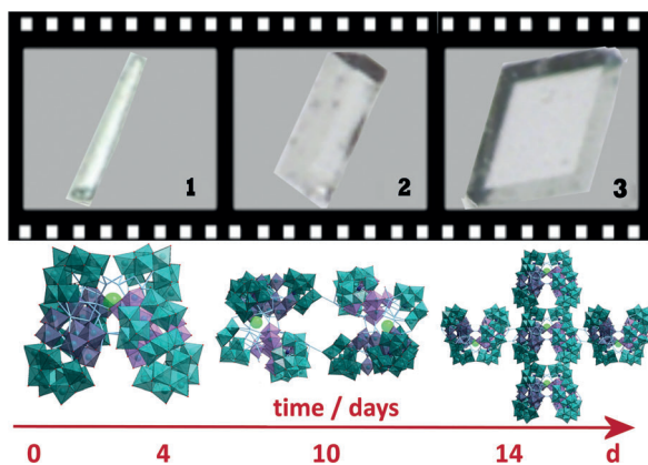
Scheme 1. Assembly pathway and time-resolved crystallization of compounds 1–3 from simple precursors to nanosized clusters and extended 3D frameworks. The \{\text{TeW}_9\} units are shown in teal/aqua polyhedra, \{\text{W}_{11}\} units are shown in lavender/blue gray polyhedra. O: red, Te: dark blue, Cl: green. The \{\text{Ag}_n\} core and linkers are shown by the pale blue wireframe. The crystal shape, size, and content changes as a function of time in solution, giving 1 to 3 in sequence.
